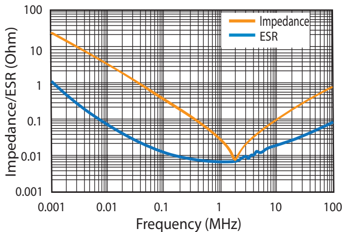
1. Impedance /ESR vs. Frequency
