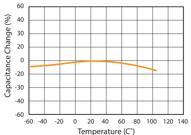
4. Capacitance vs. Temperature
