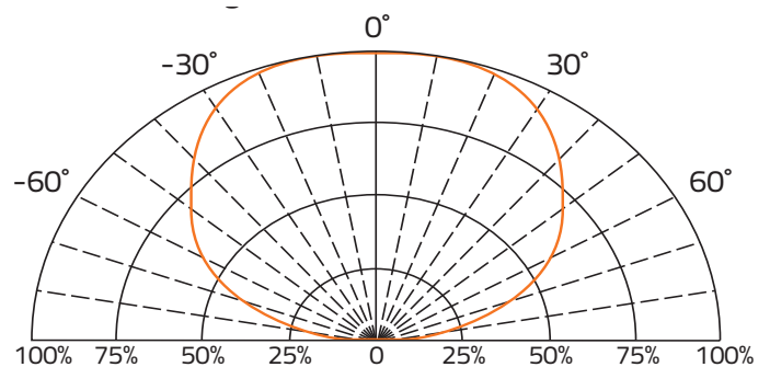
Fig. 6 Direct Radiation
